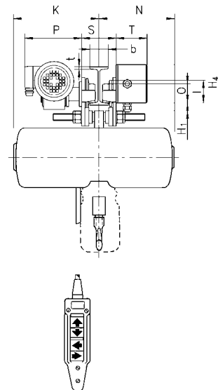
CM Lodestar, integrated electric trolley
