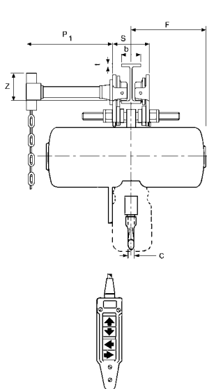
CM Lodestar, integrated push or geared trolley
