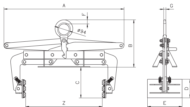
Grab with large jaw capacity
